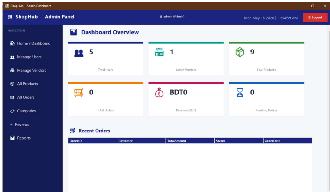
Figure 02: Admin Dashboard
