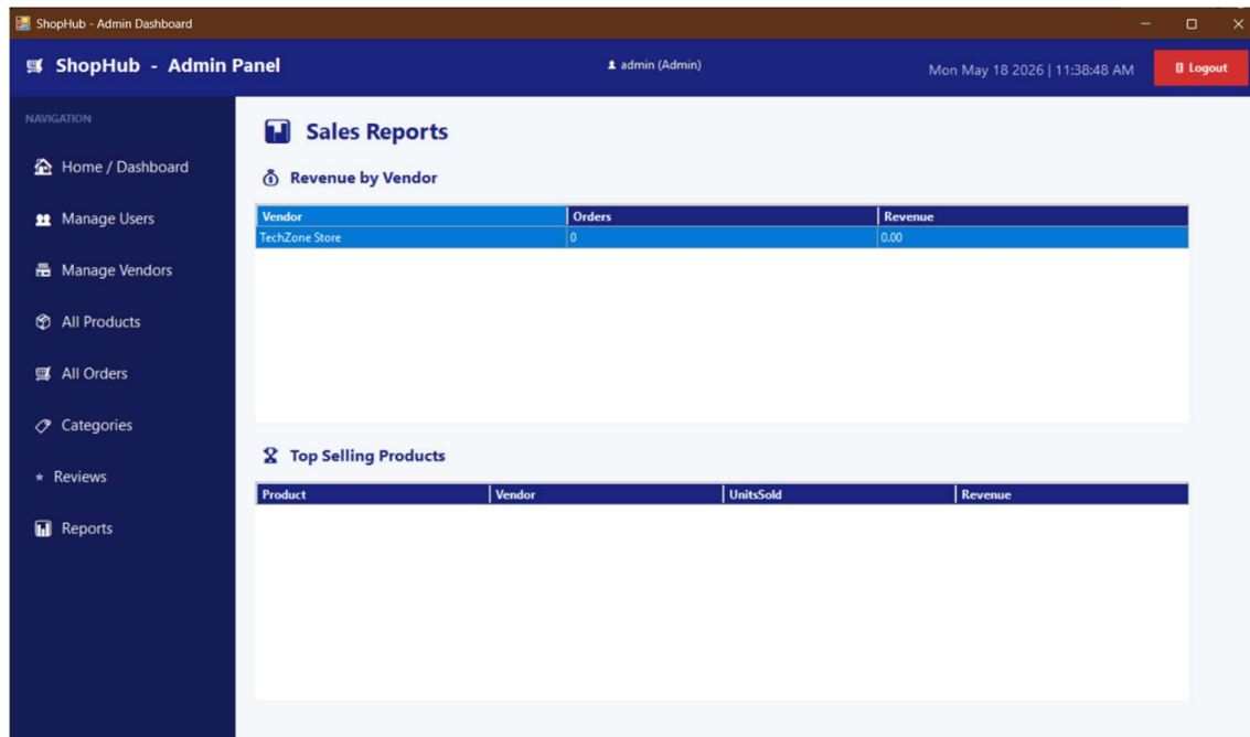
Figure 03: Admin Controls
