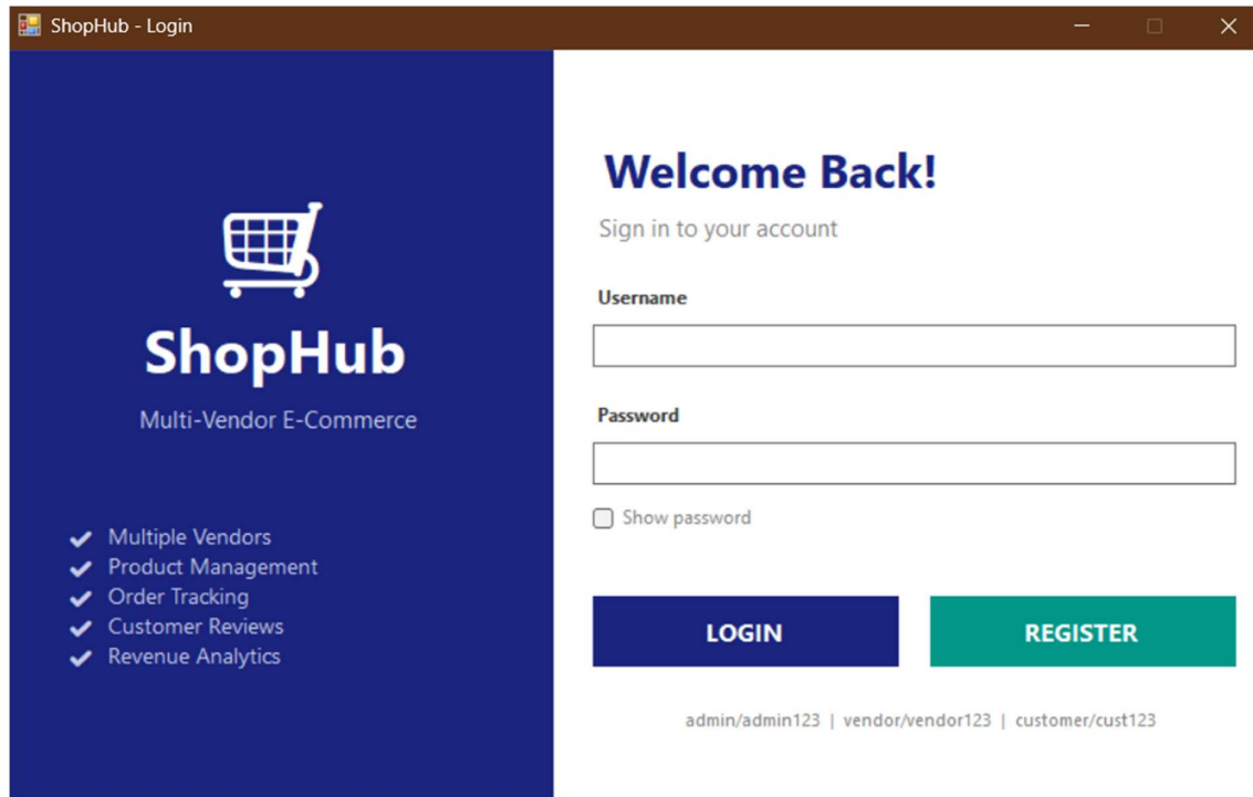
Figure 01: Login/Registration Panel
