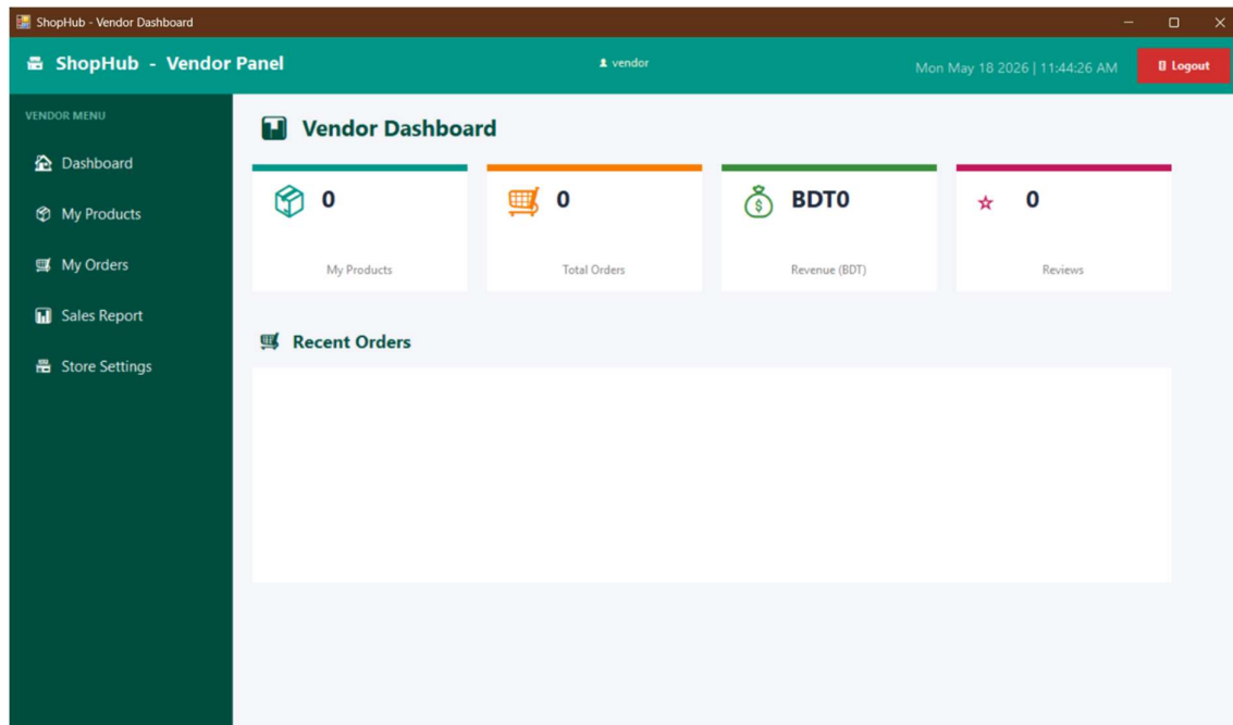
Figure 04: Vendor Dashboard
